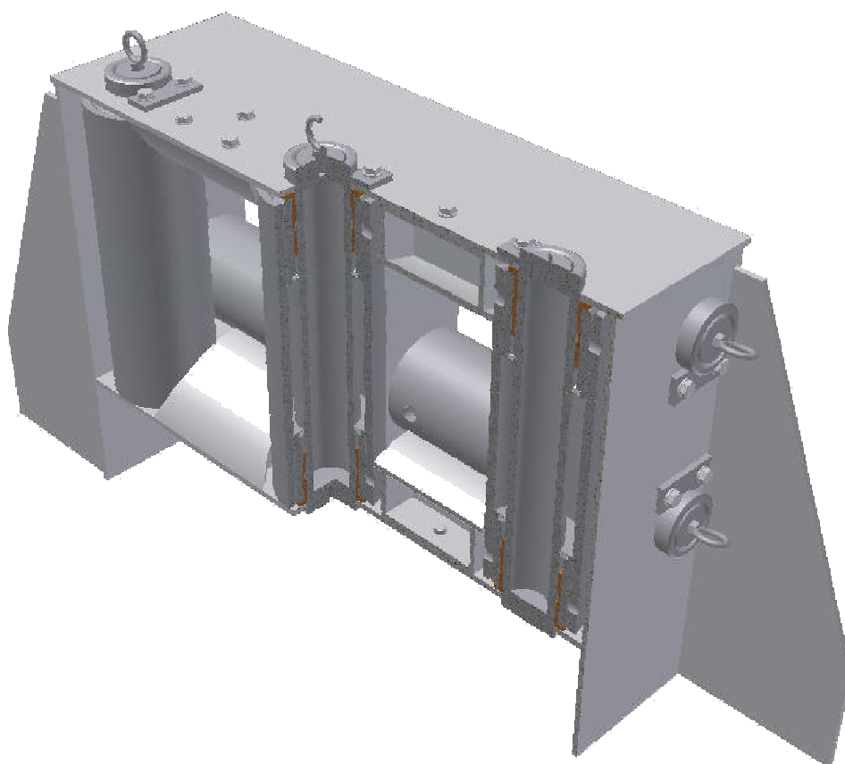
SECTION VIEW
