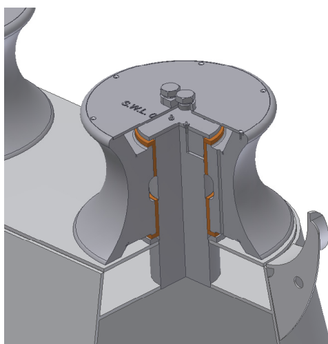
SECTION VIEW
